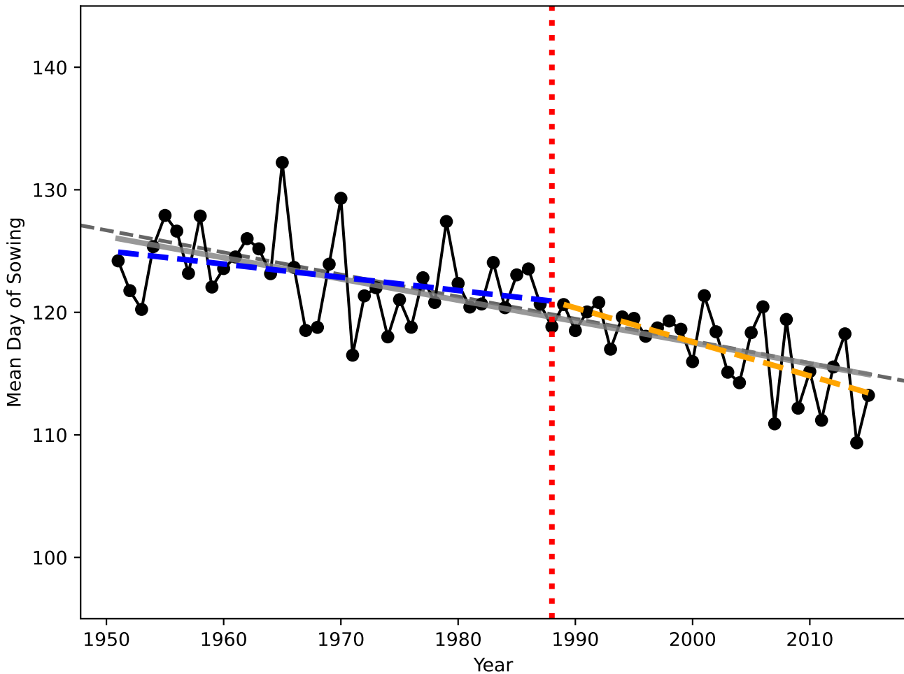
Interannual trend in the mean sowing date
